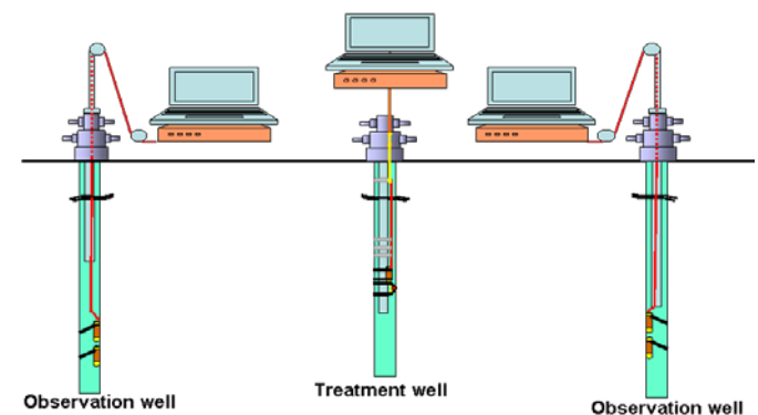
Figure 2 - Example of a survey configuration for fracturing mapping from the treatment well (where the fluids are injected at very high pressures), and observation well
