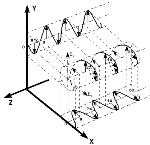
Fig. 5. Combination of two linearly polarized waves, V and H, 90^\circ out of phase. Source: (PY4ZBZ, 2008).
