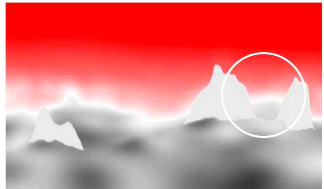
Figure 10. A section of Line B showing the depth model derived for the 2011 reprocessing. Compare with Figure 9 and with Figures 6 and 7: the salt-body definition and supra-salt velocity was significantly revised for the new model (white circles).
