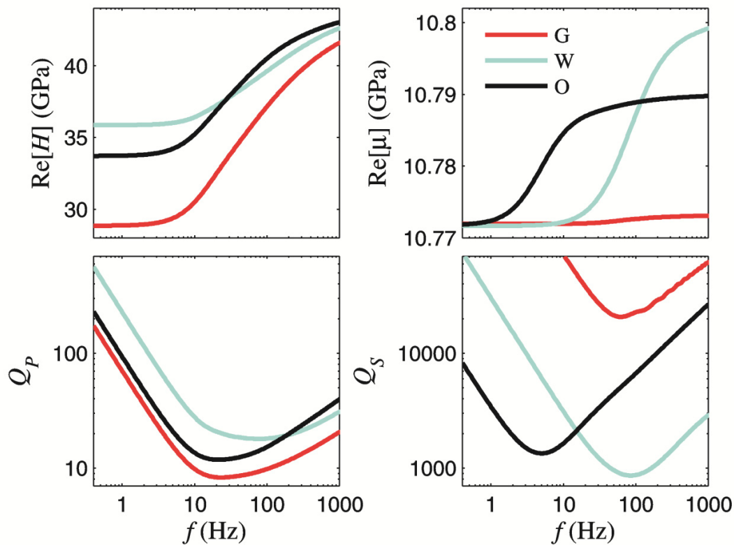
Figure 5. Numerical results for the real part of the P -wave modulus, H , the P -wave attenuation, 1/Q_p , the real part of the undrained shear modulus, \mu , and the S -wave attenuation, 1/Q_s . The petrophysical parameters are the ones from Tables 2 and 3, except K_d and \mu_d , which are 4 and 2 GPa, respectively, in the heterogeneity, and 36 and 32 GPa, respectively, in the background. So, for this figure, the less porous and permeable area (the heterogeneity) has the most compliant solid frame. The legend terms refer to the saturation in the sample: 80% gas, 20% water (G); 100% water (W); and 80% oil, 20% water (O).
