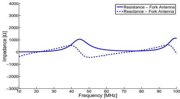
Figure 6: Simulated impedance characteristics for the Fork antenna.
