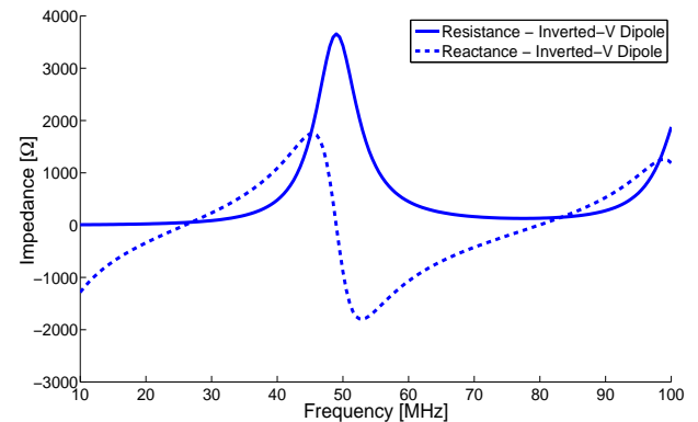
Figure 5: Simulated impedance characteristics for the Inverted-V dipole.
