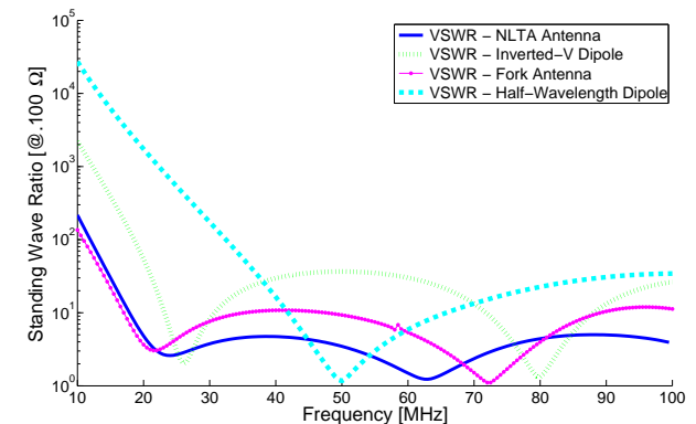
Figure 10: Standing wave ratio at the feed of the antennas NLTA (dark blue), inverted-V (light green), Fork (pink) and Half-wavelength dipole (light blue) to a normalized impedance of 100Ω.
