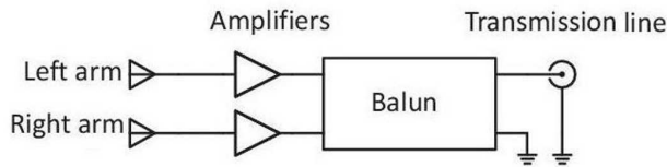
Figure 2: Basic diagram of the antenna used in the SSO.
