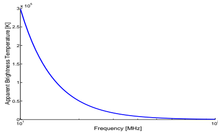
Figure 3: Apparent Brightness temperature received for a low gain antenna.
