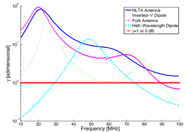
Figure 9: Comparison of \gamma = 1 (red) with \gamma calculated using the simulated VSWR for the antennas NLTA (dark blue), inverted-V dipole (light green), Fork (pink) and Half-wavelength dipole (light blue).
