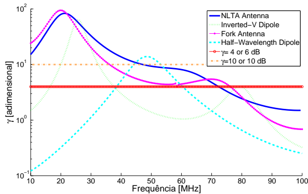
Figure 11: Comparison of \gamma = 4 (red) and \gamma = 10 (orange) with \gamma calculated using the VSWR simulated in software NEC-2 for the antennas NLTA (dark blue), inverted-V dipole (light green), Fork (pink) and Half-wavelength dipole (light blue).
