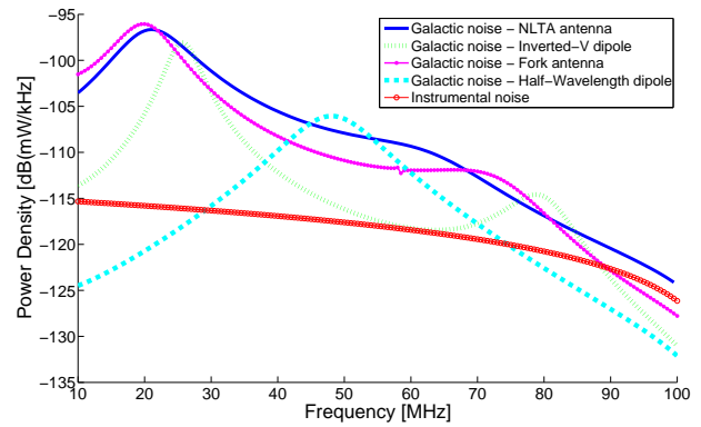
Figure 8: Power density at the receiver input to the antennas NLTA (dark blue), inverted-V dipole (light green), Fork (pink), Half-wavelength dipole (light blue) and instrumental radio noise (red).
