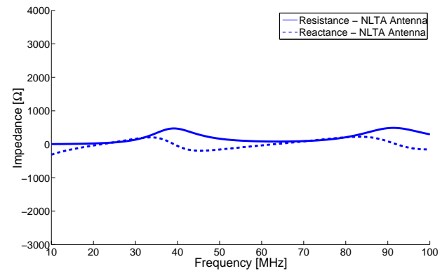
Figure 4: Simulated impedance characteristics for the NLTA antenna.
