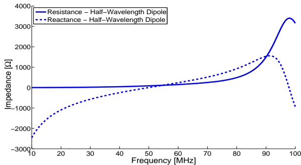
Figure 7: Simulated impedance characteristics for the Half-wavelength dipole.
