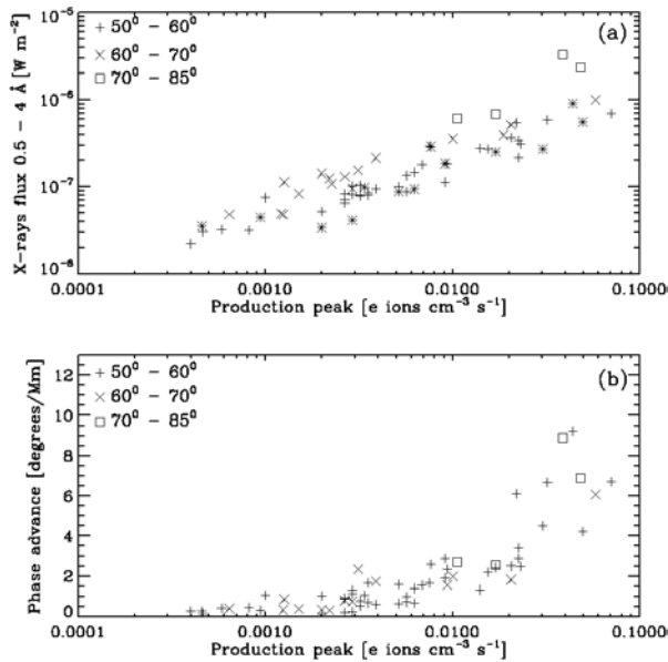
Fig. 5 – Correlations between the peak of production profile with the peak solar flux in the 0.5 – 4.0 Å (superior panel) and the SPA normalized (inferior panel).
