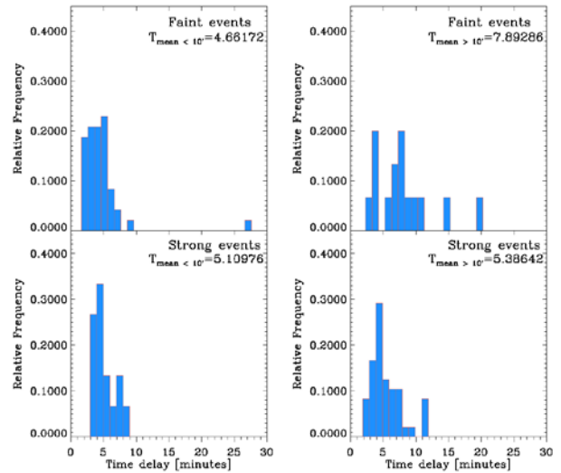
Fig. 6 – Time delay between SPA and X-rays fluxes peaks for faint and strong events.
