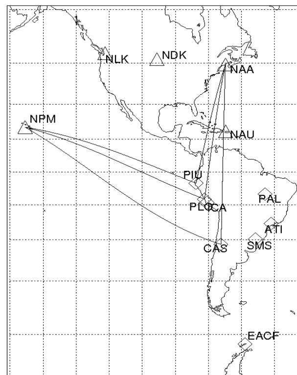
Fig.1 - The receiver bases of the SAVNET array ( \Delta ), transmitters ( \diamond ) and VLF propagation paths.
