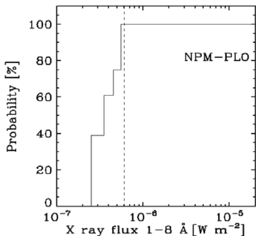
Fig. 2 – Solar flare probability detection for the NPM-PLO VLF propagation path for solar zenith angle lower than 70^\circ .
