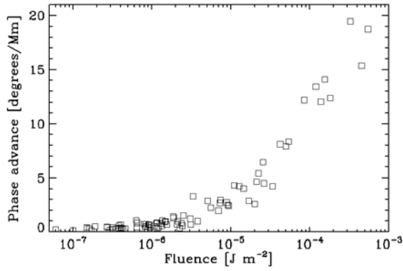
Fig. 4 - Relation between SPA amplitudes and x-ray fluence of the ray emission in the 0.5 – 2 Å.
