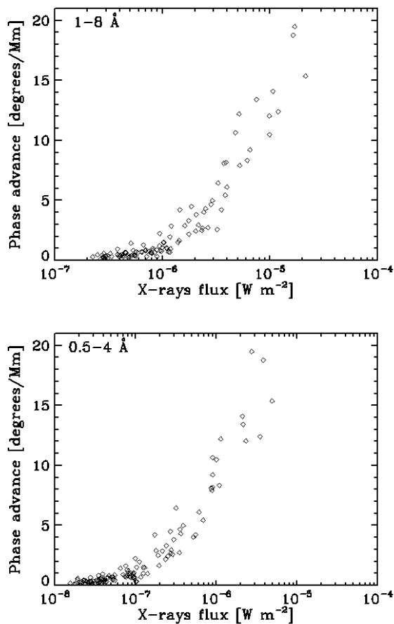
Fig. 3 - Correlation between \Phi (degrees/Mm) and GOES soft X-ray peak fluxes in the 1-8 \text{ \AA} and 0.5 - 4 \text{ \AA} excess.
