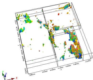
Figure 4: MVI for the Crixas area. Vertical exaggeration 2, cell size x=190 m; y=190 m and initial value for z= 25 m. Results clipped to Amplitude = 0.003.
