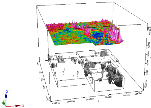
Figure 9: Amplitude of the Analytic signal with color and relief in 3D over results of Magnetization Vector Inversion in gray for the Crixas areas 2, 3 and 5. Projected and perpendicular components
