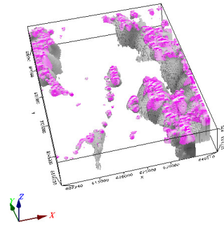
Figure 11: Results of the Magnetization Vector Inversion for Crixas area 5. Comparison of MVI total magnetic field inversion results in gray with MVI residual magnetic inversion in magenta.
