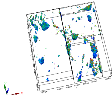
Figure 3: Susceptibility inversion for the Crixas area. Vertical exaggeration 2, cell size x=190 m; y=190 m and initial value for z= 25 m. Results clipped to 0.005 SI units.
