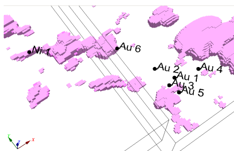
Figure 5: Voxel result from MVI inversion for the Crixas area 2 and 3. Projected and Perpendicular components combined with location and identification of the mine locations as provided by DNPM.
