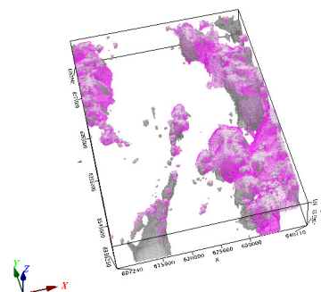
Figure 6: Susceptibility and Magnetization Vector Inversion for the Crixas area 5. No vertical exaggeration, cell size x=190 m; y=190 m and z initial = 25 m. Susceptibility in gray clipped to 0.04 and projected and perpendicular components of the magnetization vector in magenta filtered using the amplitude component.
