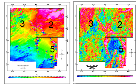
Figure 2: Merged TMI (left) and Analytic Signal (right) with the survey outlines for Areas 2,3 and 5.
