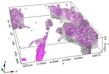
Figure 10: Results of the Magnetization vector Inversion for Crixas area 5. Comparison of MVI non-constrained results in gray with one reweighting iteration in magenta.
