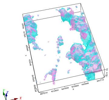
Figure 7: Results of the Magnetization Vector Inversion for Crixas area 5. No vertical exaggeration, cell size x=190 m; y=190 m and initial z = 25. Projected component in magenta and perpendicular component in cyan.
