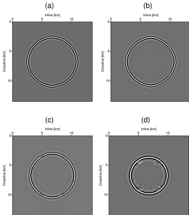
Figure 6: Corresponding slices of Figure 3 with approximate Li correction (38) using angles extracted from the propagating wavefield with smoothing.
