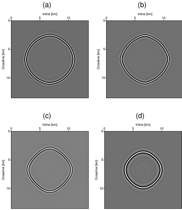
Figure 3: Horizontal slices through the impulse response of FD migration without Li correction in a homogeneous medium at the depths (a) 480 m, (b) 960 m, (c) 1920 m, and (d) 2880 m.
