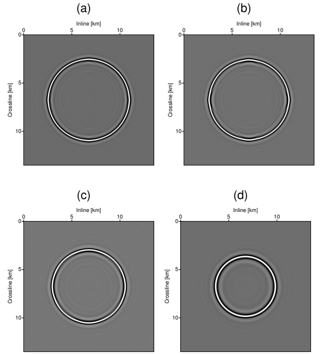
Figure 4: Corresponding slices of Figure 3 after approximate Li correction (38) using the angles calculated from the grid position.
