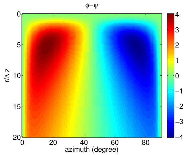
Figure 2: Stationary value of the difference \phi - \psi as obtained by solving system (33-34) by means of Newton's method.
