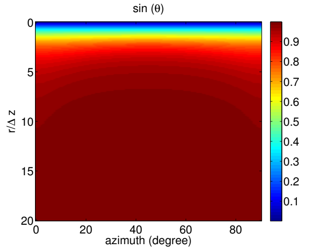
Figure 1: Stationary value of \sin \theta as obtained by solving system (33-34) by means of Newton's method.
