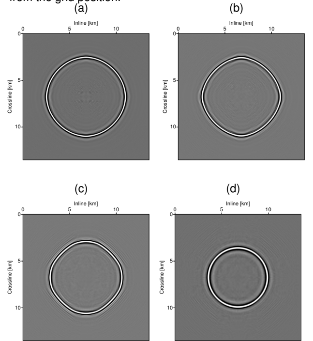
Figure 5: Corresponding slices of Figure 3 with approximate Li correction (38) using angles extracted from the propagating wavefield.
