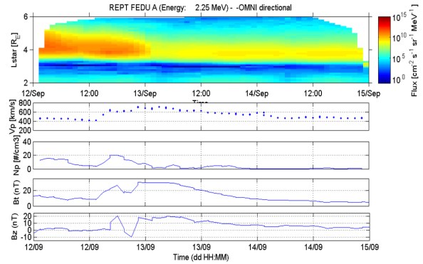
Figure 1: Radiation belt dropout observed from Van Allen Probes data on the top panel, the following panel are the solar wind velocity, density, total magnetic field and north-south component.
