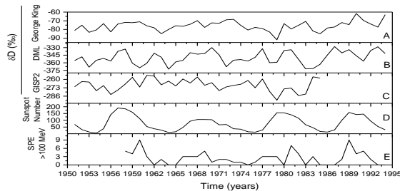
Figure 1 – The \delta D Annual average time series from: Antarctica - George King island (A), and Dronning Maud Land (B); Greenland - GISP2 (C); Suspot Number (D); SPE ( E_p > 100 MeV)(E) time series.
