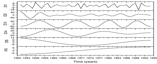
Figure 2 – Wavelet decomposition bands for the Sunspot Number time series 1950-1994.
