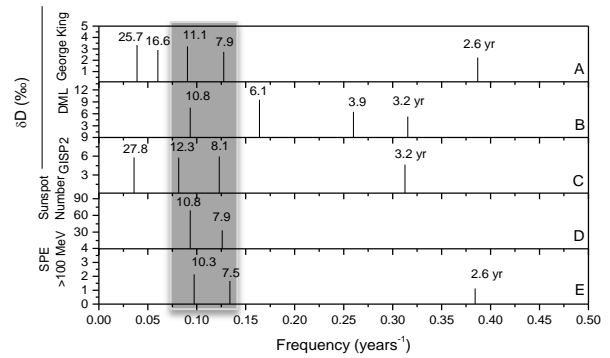
Figure 3 – Amplitude spectrum for δD Annual average time series from George King island (A), and Dronning Maud Land (B), GISP2 (C), Sunspot Number (D), and SPE (E p > 100 MeV) (E).
