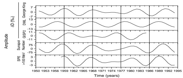
Figure 4 – Signal of 7+12 years reconstruction from time series.
