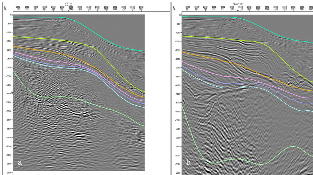
Figure 6: a) Horizons in time and b) horizons converted to depth by vertical ray with the velocity model created by cokriging the interval velocity of the wells with the seismic in the region of the Foz do Amazonas Basin.
