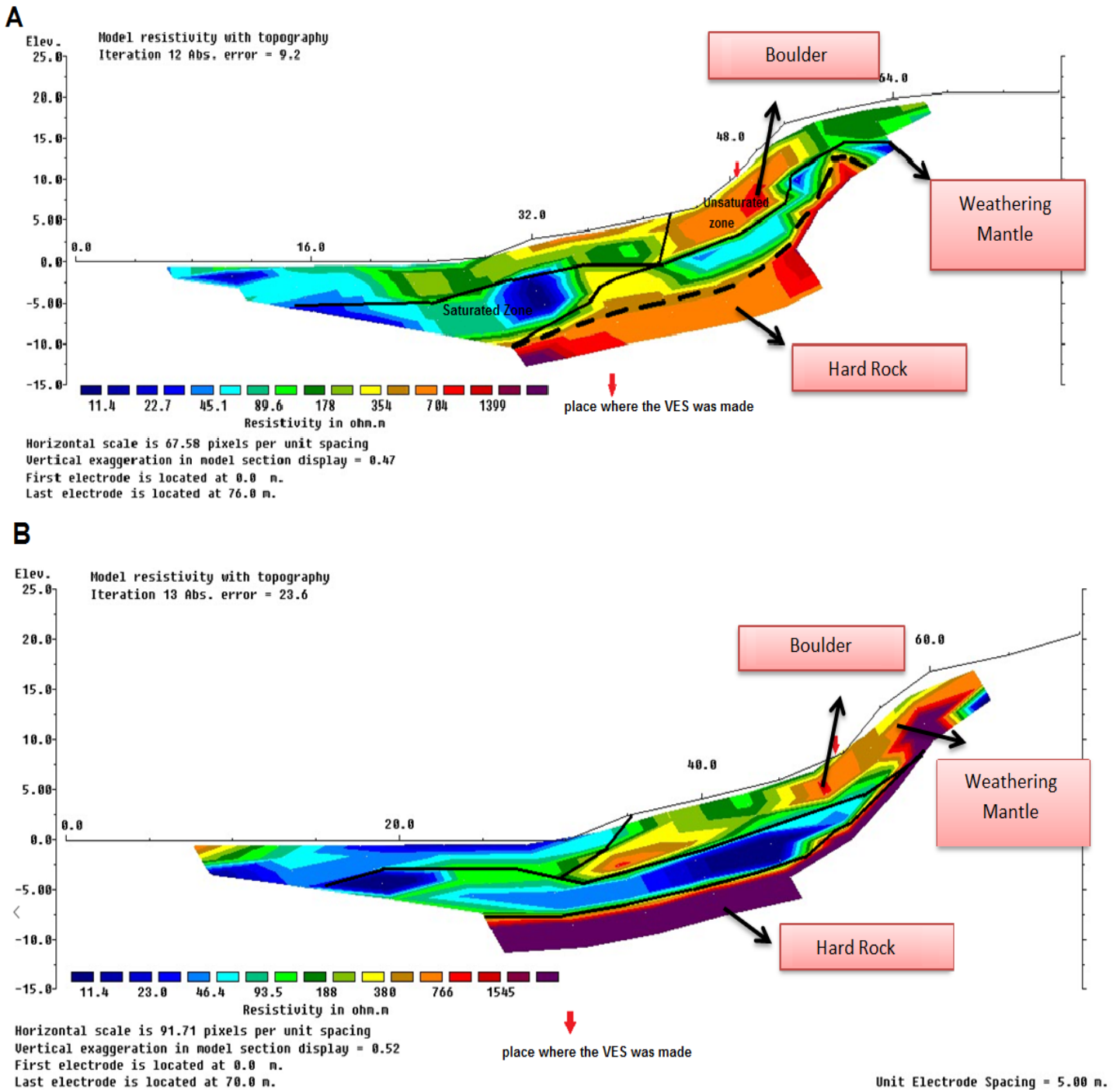
Figure 2: (a) Inverted 2D resistivity model ( M_{1INV} ) for the ERT I, using the dipole-dipole array. The spacing between the dipoles was 4 m. This model presented the RMS error, between the calculated and the observed data, of 9.2 % (b) Inverted 2D resistivity model ( M_{2INV} ) for the ERT I, using the dipole-dipole array. The spacing between the dipoles was 5 m. This model presented the RMS error, between the calculated and the observed data, of 23.6 %.
