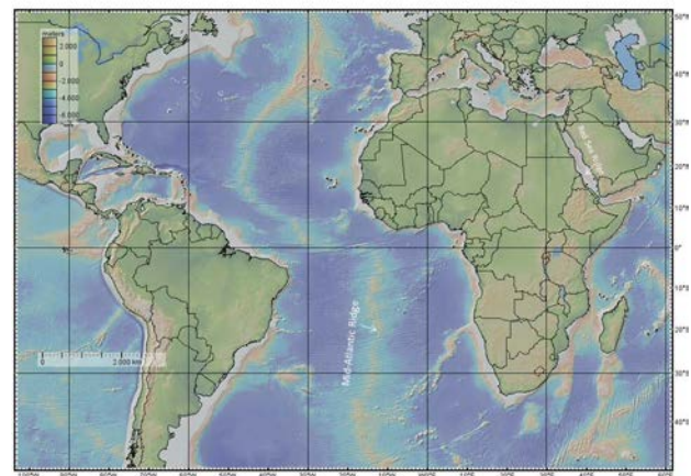
Figure 1: Continental margin basins in the South and North Atlantic and in the Red Sea.
