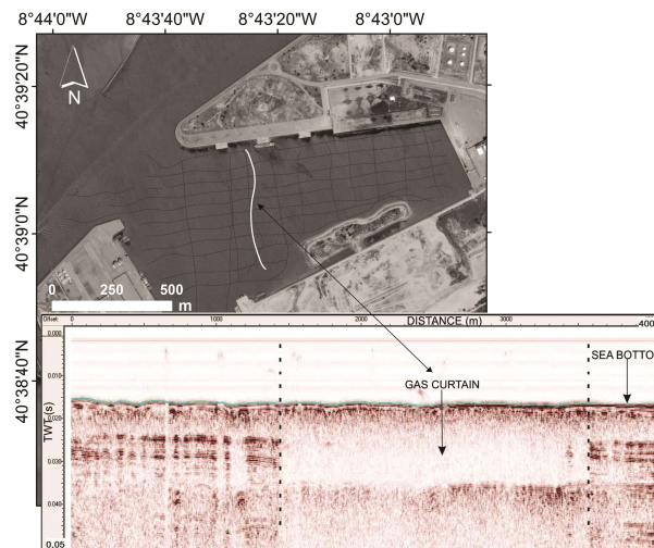
Figure 3 – Seismic profile of line TNC12 with evidence of gas accumulation.
