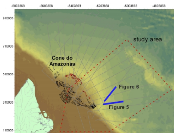
Figure 3: Bathymetric map of the Foz do Amazonas basin showing the location of the study area and the dataset (3.5 kHz profiles) used on this project.
