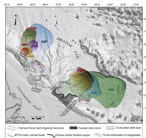
Figure 1: Simplified map illustrating Amapá Megalide Complex and the Para-Maranhão Megalide Complex areas and structural domains on the upper slope (after Reis et al. , 2016).
