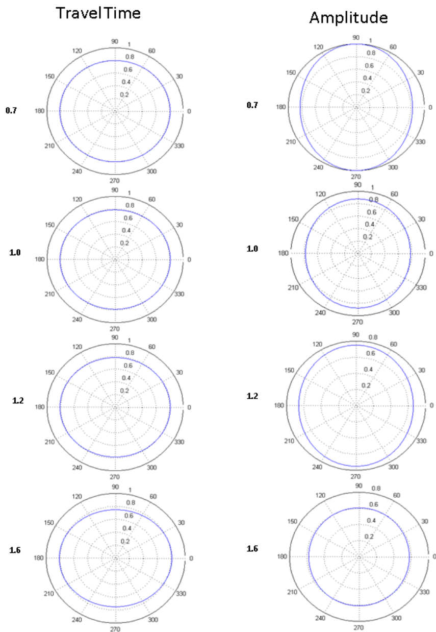
Figure 6 - Azimuthal variations of P-wave travel-time (left) and amplitude (right) at the top of the fractured layer, with the offset to depth ratios of 0.7, 1.0, 1.2 and 1.6.
