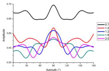
Figure 9 - Amplitude variation with azimuth for offset-depth ratio of 0.7 (black), 1.0 (red), 1.2 (blue), 1.6 (green) and 2.0 (pink).
