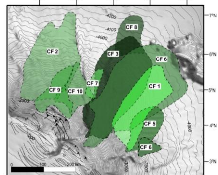
Figure 2: The Central Amazon Fan Megaslides Complex and structural domains localized on the upper slope (modified from Silva et al. , 2016). CF1 to CF10 are stacks of megaslides in late Neogene-Quaternary sedimentary succession.
