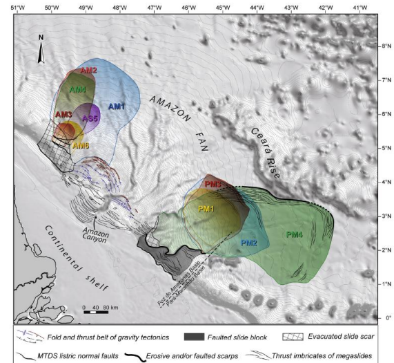
Figure 1: Simplified map illustrating Amapá Megaslide Complex and the Para-Maranhão Megaslide Complex areas and structural domains on the upper slope (after Reis et al. , 2016).
