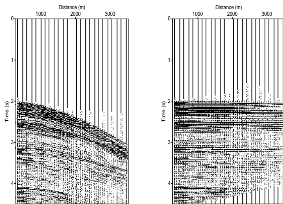
Figure 4: CMP 450 before (left), and after the NMO correction (right).
