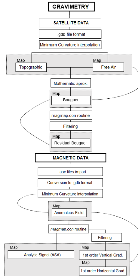
Figure 4: Flowchart of gravimetric and magnetic processing routine.
