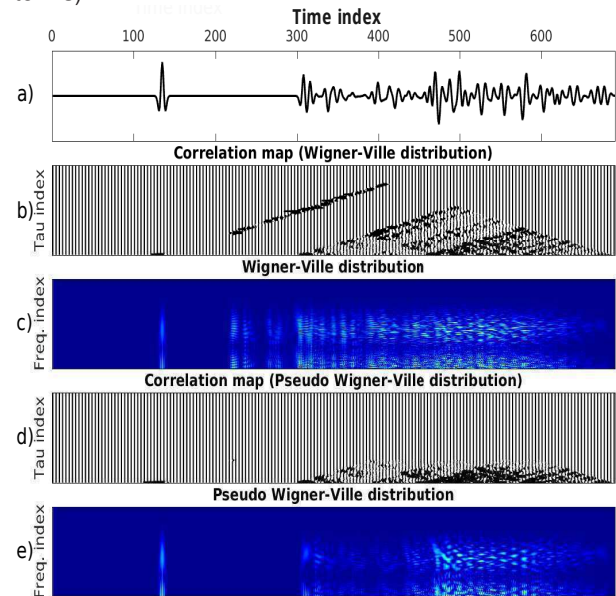
Figure 5: (a) Seismic trace without noise. Distributions: (b) Correlation map of the Wigner-Ville. (c) Wigner-Ville. (d) Correlation map of the Pseudo Wigner-Ville. (e) Pseudo Wigner-Ville.
