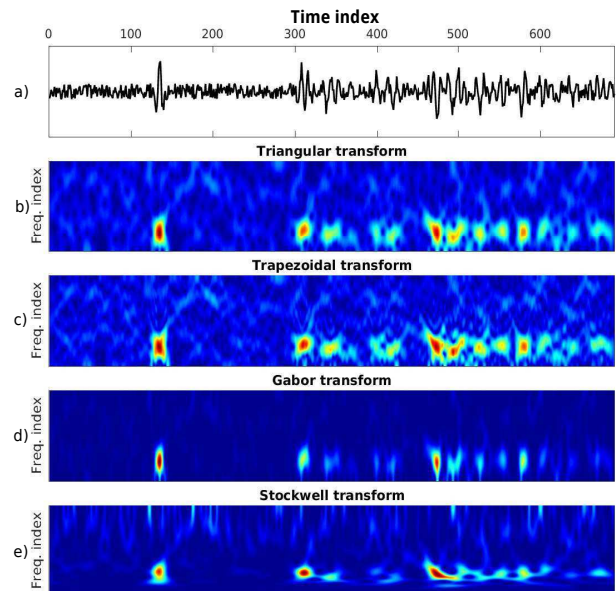
Figure 8: (a) Seismic trace with noise. Windows and Fourier transform: (b) Triangular. (c) Trapezoidal. (d) Gabor. (e) Stockwell.
