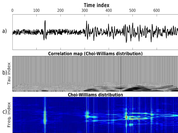
Figure 10: (a) Seismic trace with noise. Distributions: (b) Correlation map of the Choi-Williams. (c) Choi-Williams.
