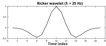
Figure 2: Ricker wavelet.
