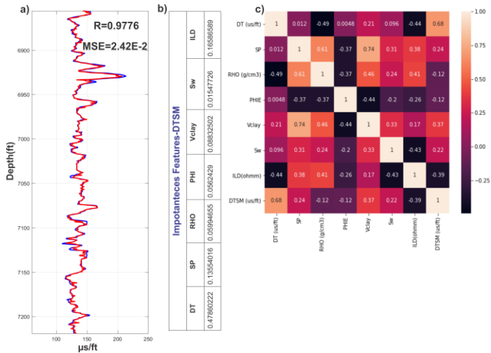
Figure 4. Estimation of DTSM using Random Forest. a) We have a correlation factor of R=0.9776 between these two parameters and MSE=2.42 \times 10^{-2} , b) Importance Features, and c) correlation matrix.
