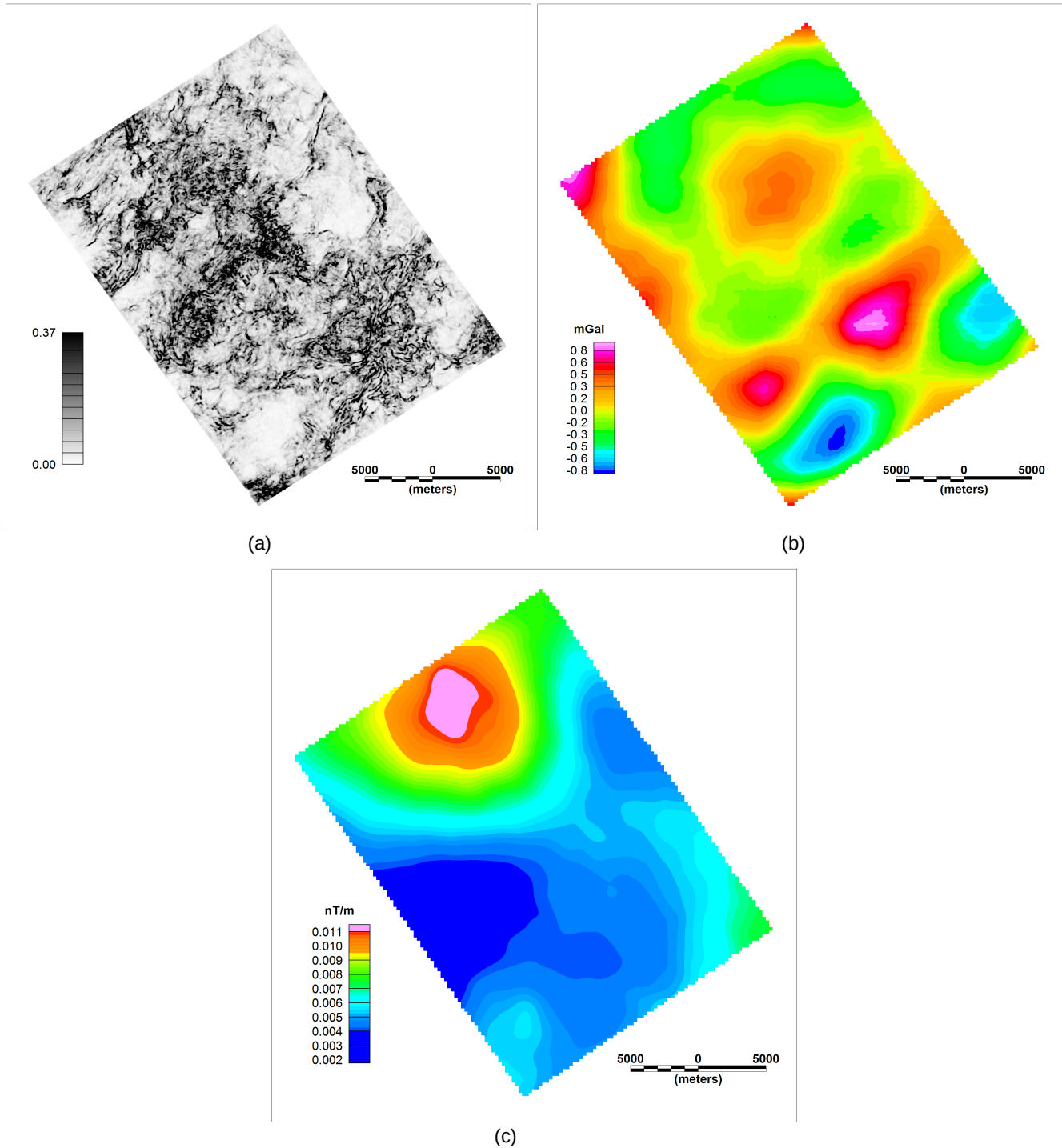
Figure 2 – Anomalies selected for construction of the multiphysics anomaly map in block BMC-33, Campos Basin, Brazil. In the seismic discontinuity in (a) the dark areas were interpreted as indicative of volcanic rocks. The gravity residual in (b) shows positive anomalies, usually related to high density rocks, which can indicate presence of igneous rocks. The strong magnetic anomaly in the amplitude of the analytic signal in (c) may also represent the response of volcanic rocks.
