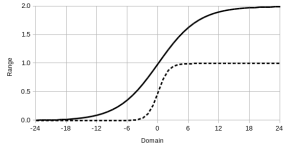
Figure 3 – Example of logistic functions. In dashed line is the standard sigmoid function while the modified logistic function is shown by the solid line.
