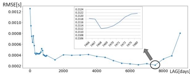
Figure 11: Each point on the graph represents the error of a simulation performed for different lags for the 500-days forecast. The best model found was AR (7468) with RMSE error of 2,112 \times 10^{-4} seconds.
