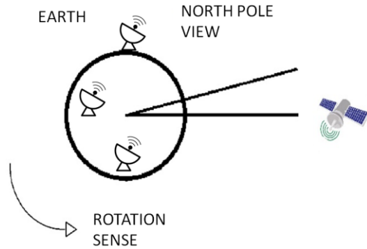
Figure 3. This is the view from the north pole of planet Earth. The arrow represents the direction of the Earth's rotation, while the lines represent a small displacement on Earth of milliseconds more, this can generate a large displacement in space (the figure is not scaled).
