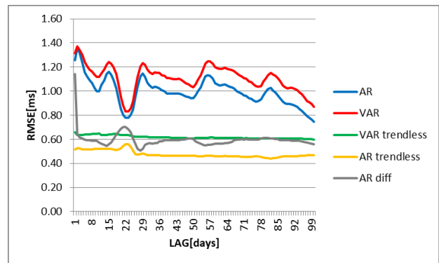
Figure 14: When using lags between 1 and 100, it is easy to compare which one has better performance. The graph shows the variation of the error of the LOD forecasts in relation to the lag used.
