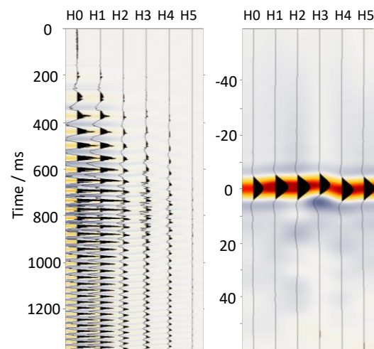
Figure 3 - Snippet of observed 5s sweep recorded by H0-H5 showing the first 1.4 s (left) and after deconvolution (right) using the forward modelled trace.
