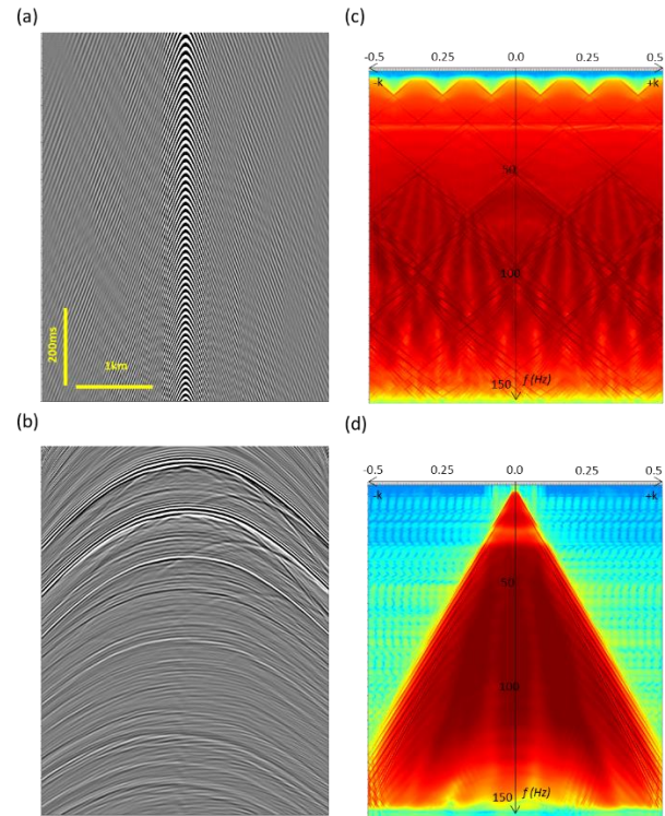
Figure 5 – (a,c) Raw synthesized marine vibrator data using an array of one high-band unit and one low-band unit including phase encoding, source ghost and source motion and (b,d) data after full processing. Wavenumbers in (c) are normalized, scaled by the trace spacing 12.5m and for (d) 6.25m.
