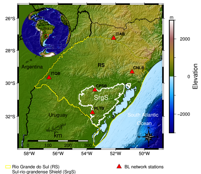
Figure 1 - Topo-altimetric location map (TOPODATA - Brazil, 2008) with location of the permanent seismic stations (red triangles) and with the Srg region outline (white polygon).
