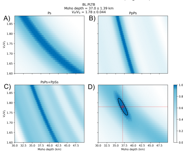
Figure 4 - H-k stacking of PLTB station using P wave speed of 6.4 km/s. (A) The converted Ps wave. (B) The multiple PpPs. (C) The multiple PsPs+PpSs. (D) result of the estimation.
