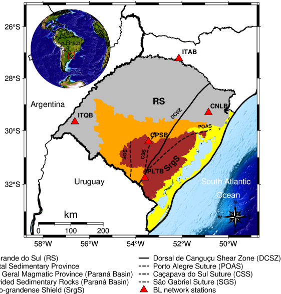
Figure 2 - Map of the geological context of the study area. Modified from Viero and Silva (2010).
