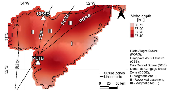
Figure 8 - Map of the estimated depth of the SrgS Moho with the limits of the SrgS (white polygon), the main suture zones (dashed black line), the seismic stations used (white triangles). The tectonic domains are according to Fernandes et al. (1995).
