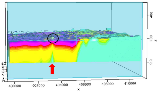
Figure 11- Cut at (Y= 9565400) near the epicenter.
