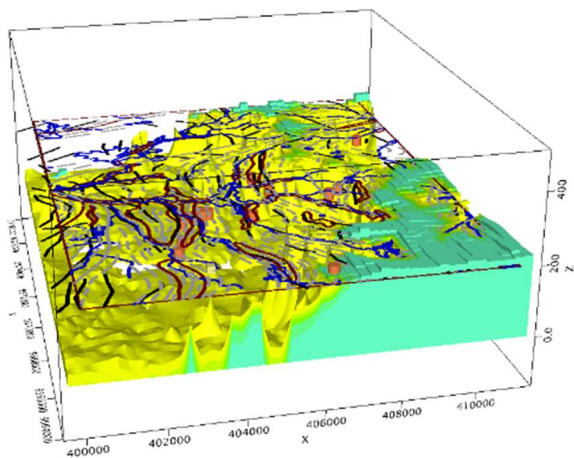
Figure 6- Voxel result of the inversion (0.0008-0.0011 S/m ).
