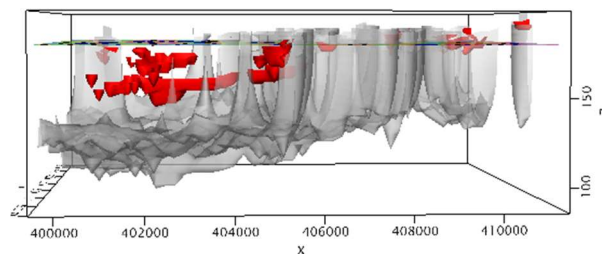
Figure 9- Voxel of the red (conductive) and the gray (resistive) isosurfaces.
