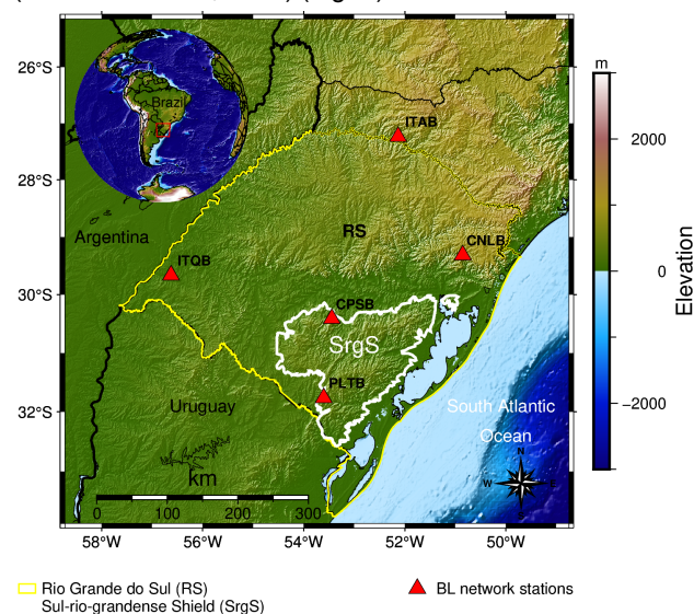
Figure 1 - Topo-altimetric location map (TOPODATA - Brazil, 2008) with location of the permanent seismic stations (red triangles) and with the SrgS region outline (white polygon).
