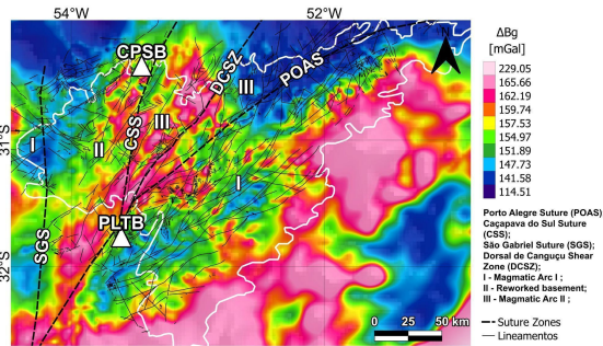
Figure 7 - \Delta Bg map of the SrgS with the limits of the SrgS (white polygon), the main suture zones (dashed black line), the main lineaments (thin black line) and the seismic stations used (white triangle). The tectonic domains are according to Fernandes et al. (1995).
