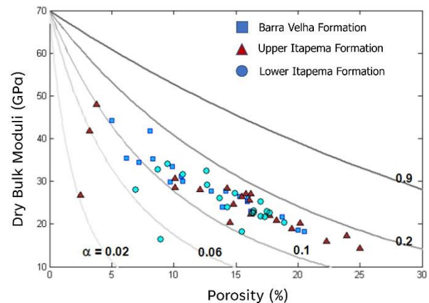
Figure 3 – Rock-physics template modeling of the Differential Effective Medium (DEM) in calcite-dominated samples. The lines represent the aspect ratios (modified from Morschbacher, 2016).
