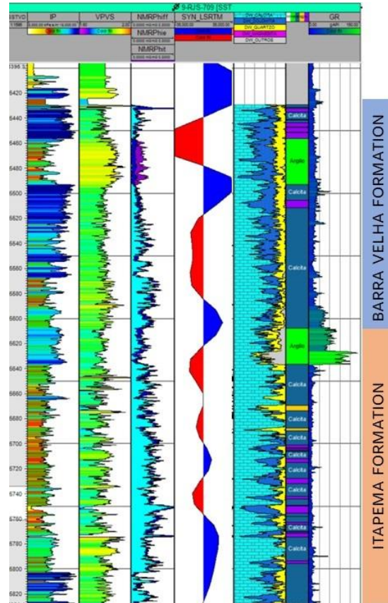
Figure 2 – Well 9-RJS-709. From left to right: acoustic impedance, compressional-to-shear velocity ratio ( V_p/V_s ), NMR porosity, the synthetic seismic, the accumulative lithochemochemistry log, the interpretation of predominant mineralogical facies, and gamma ray log. Key color: silica-rich (yellow), dolomite-rich (purple), calcite-rich (blue), clay-bearing (green) facies.
