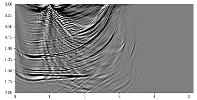
Figure 5: (a). Single-shot RTM. (b) Single-shot RTM with CNN-based preconditioning.
