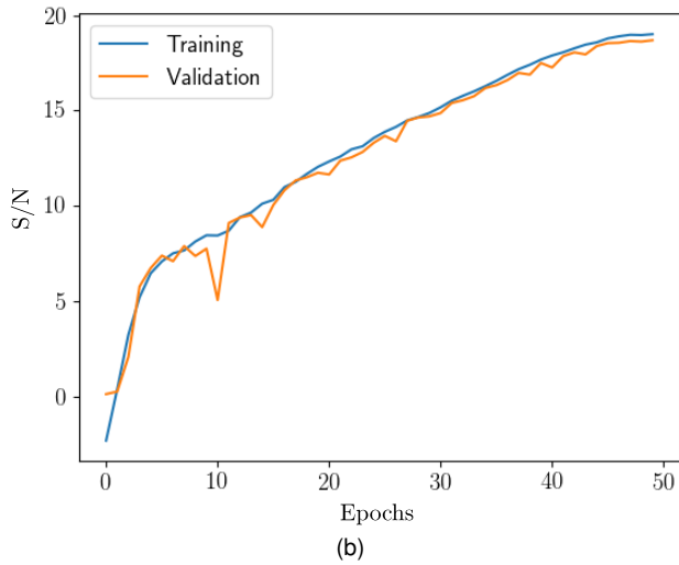
Figure 3: (a) The normalized training and validation loss functions versus the number of epochs. A similar pattern between both curves indicates that our method does not suffer from the overfitting problem. (b) Evolution of the signal-to-noise ratio (dB) = 10 \times \log_{10} \frac{\|\mathbf{d}_{\text{mig}}\|_2^2}{\|\mathbf{d}_{\text{mig}} - \mathbf{d}_{\text{obs}}\|_2^2} , versus the number of iterations to measure reconstruction accuracy.
