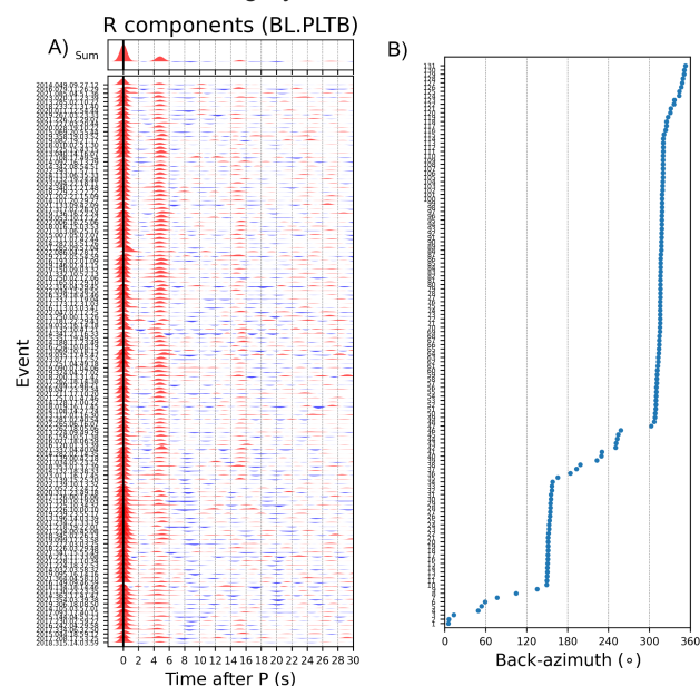
Figure 2 -Receiver Functions selected for the PLTB station. (A) The Radial component. (B) The backazimuth in degrees.
