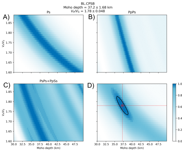
Figure 5 - H-k stacking for station CPSB using P wave speed of 6.4 km/s. (A) The converted Ps wave. (B) The multiple PpPs. (C) The multiple PsPs+PpSs. (D) Result of this estimation.
