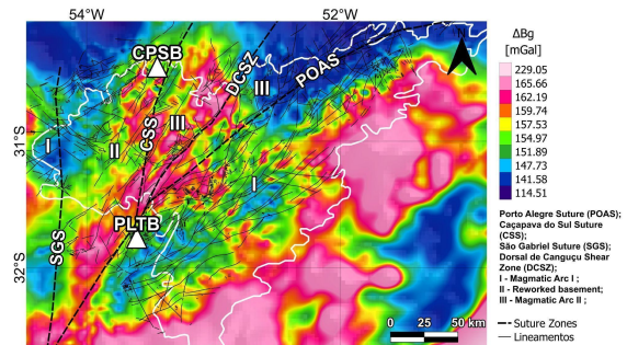
Figure 6 - \Delta Bg map of the SrgS with the limits of the SrgS (white polygon), the main suture zones (dashed black line), the main lineaments (thin black line) and the seismic stations used (white triangle). The tectonic domains are according to Fernandes et al. (1995).
