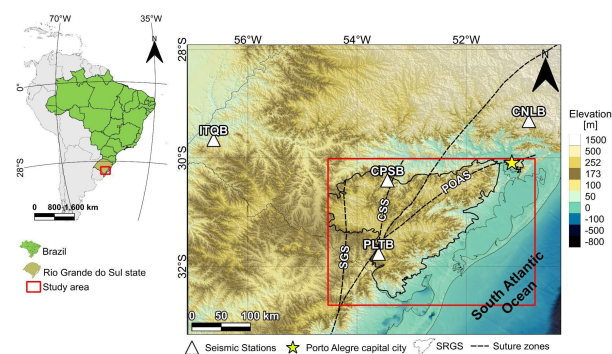
Figure 1 - Topo-altimetric location map (TOPODATA - Brazil, 2008) with location of the permanent seismic stations (white triangles) and with the Srg region outline (black polygon). Modified from Viero and Silva (2010). The abbreviations are: Porto Alegre Suture (POAS); Caçapava do Sul Suture (CSS); São Gabriel Suture (SGS); Dorsal de Canguçu Shear Zone (DCSZ).
