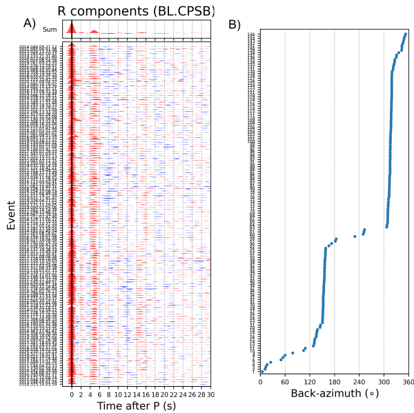
Figure 4 - Receiver functions selected for the CPSB station. (A) The Radial component. (B) The back-azimuth in degrees.
