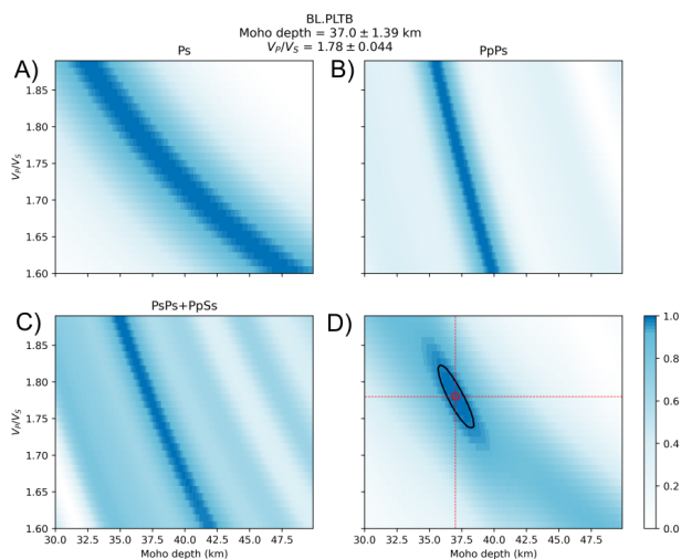
Figure 3 - H-k stacking of PLTB station using P wave speed of 6.4 km/s. (A) The converted Ps wave. (B) The multiple PpPs. (C) The multiple PsPs+PpSs. (D) result of the estimation.
