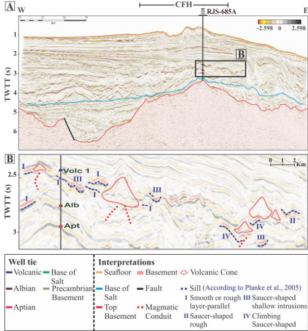
Figure 2: (A) Seismic section in the CFH drilled by the exploratory well 1-RJS-685A. The location can be seen in Figure 1. (B) Zoom view of previous seismic section displaying vents, sills and magmatic conduits.
