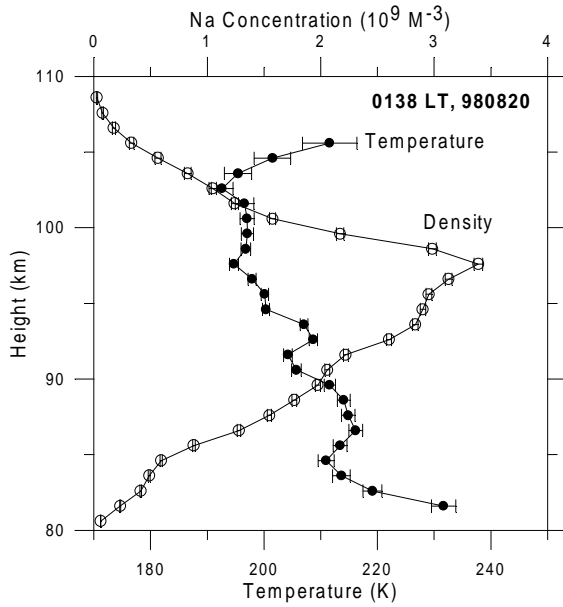
Fig. 2 As for Figure 2, but 3 hours later.
