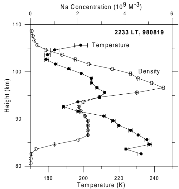
Fig. 1 Vertical distributions of sodium concentration and temperature averaged over 30 minutes centered on 2233 LT, August 19, 1998.
