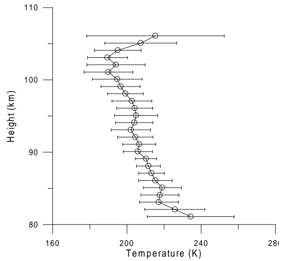
Fig. 3 Average temperature profile for all measurements, July - October, 1998.
