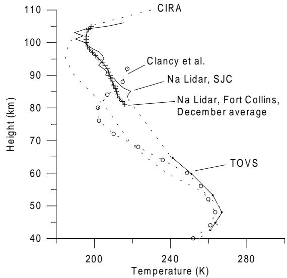
Fig. 4 Comparison between mean temperature profile for 23° S (SJC) and other profiles.
