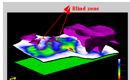
Fig. 7 Amplitude map with "blind zones" on the target horizon based on CSP shooting.
