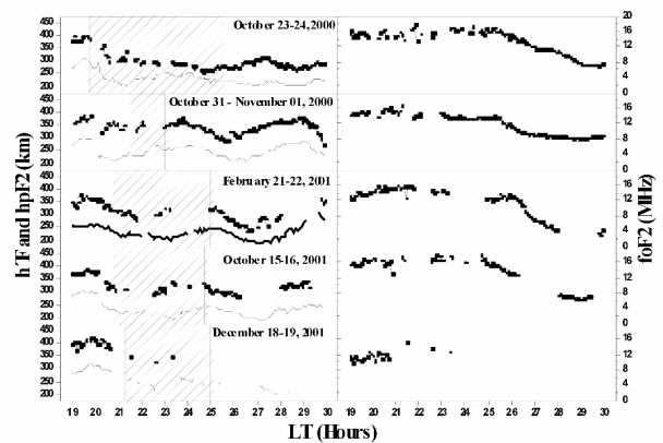
Figure 4 - F region minimum virtual height ( h'F – upper line) and virtual height at 0.834 of foF2 ( hpF2 – lower line) variations (left hand side), and critical frequency (foF2) variations (right hand side), observed at low-latitude station São José dos Campos on five nights: October 23-24, 2000; October 31-November 01, 2000; February 21-22, 2001; October 15-16, 2001 and December 18-19, 2001. The hatched portions indicate the period of imaging observations.
