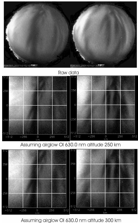
Figure 1 - All-sky airglow images at OI 630.0 nm observed at São José dos Campos, Brazil, on October 15, 2001. The local times are 21:01:45 (left) and 21:30:46 (right). The images are raw (top) and linearized assuming emission peak altitudes of 250 km (middle) and 300 km (bottom). The linearized images are divided in 16 cells, with the top left cell being (1,1).
