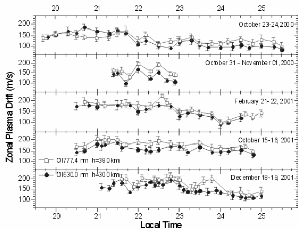
Figure 3 - Zonal plasma drift velocities inferred from the OI 630.0 nm and OI 777.4 nm emissions all-sky observations using linearized images assuming emission peak altitudes of 300 km and 380 km, respectively, and displacements of the western walls of the intensity depletion bands (dark structures as shown in Figures 1 and 2).
