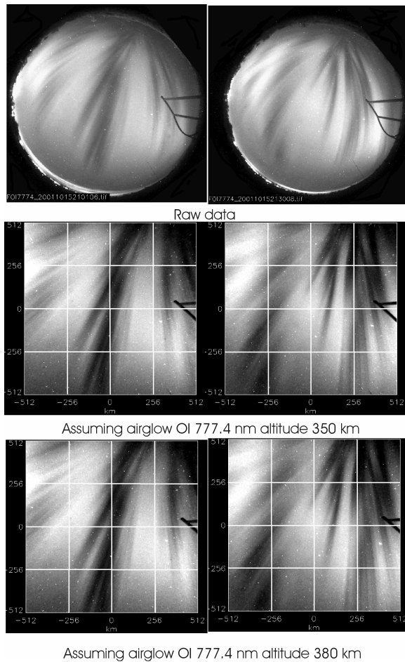
Figure 2 - All-sky airglow images at OI 777.4 nm observed at São Jose dos Campos, Brazil, on October 15, 2001. The local times are 21:01:06 (left) and 21:30:08 (right). The images are raw (top) and linearized assuming emission peak altitudes of 350 km (middle) and 380 km (bottom).
