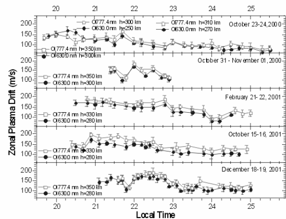
Figure 5 - Zonal plasma drift velocities recalculated for the OI 630.0 nm and OI 777.4 nm emissions using the displacements of the western walls of the intensity depletions (dark structures of Figures 1 and 2), for linearized images assuming different emission peak altitudes based on the simultaneous ionospheric sounding observations.
