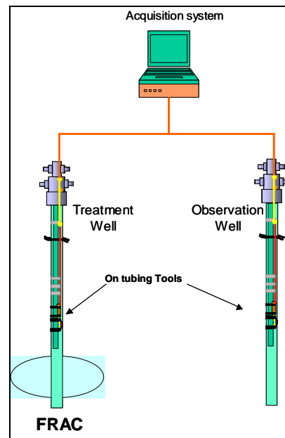
Figure 3 - Survey configuration for the second fracturing job. Treatment well (where the fluids are injected at very high pressures) is well A, observation well is well B.
