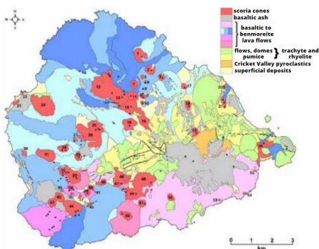
Figure 3. Geological map of Ascension Island
