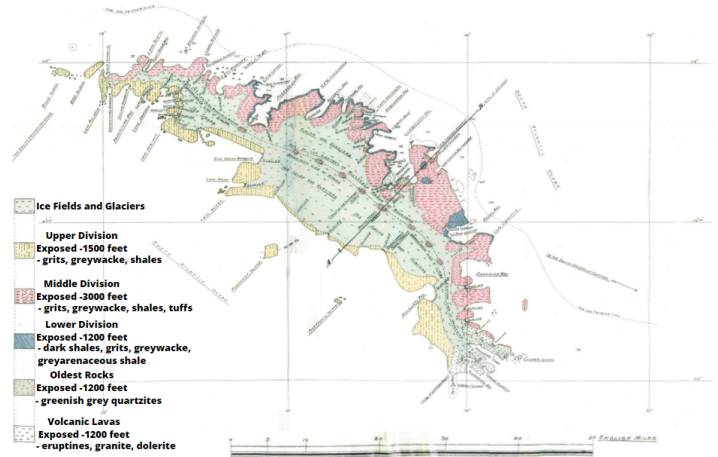
Figure 4. Geological map of South Georgia(KEP)
