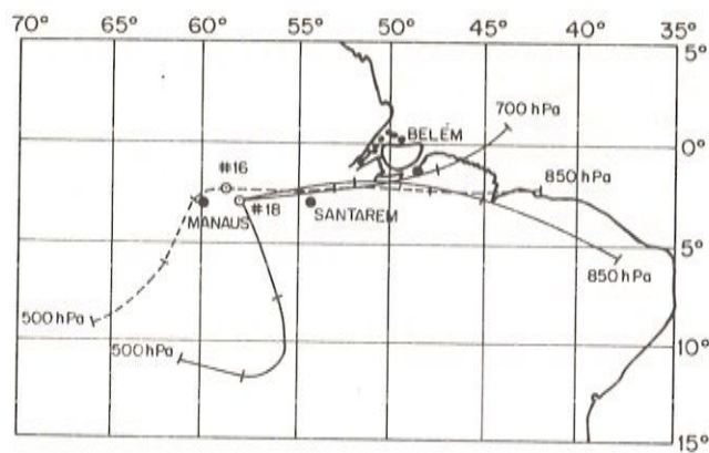
Figure 4. 3 day isobaric back trajectories for flight #16 and #18.
