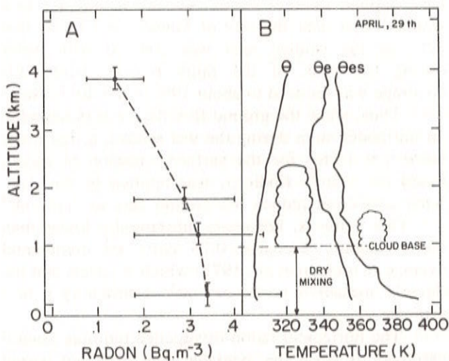
Figure 2. Flight #16 - a) radon versus geometric altitude, b) thermodynamic variable: \theta potential temperature; \theta_e = equivalent potential temperature; \theta_{es} saturated equivalent potential temperature.
