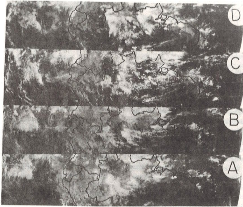
Figure 7. Infrared satellite images corresponding to flights #12 and #13. A) 6:00 UTC; B) 12:00 UTC; C) 18:00 UTC; D) 0:00 UTC
