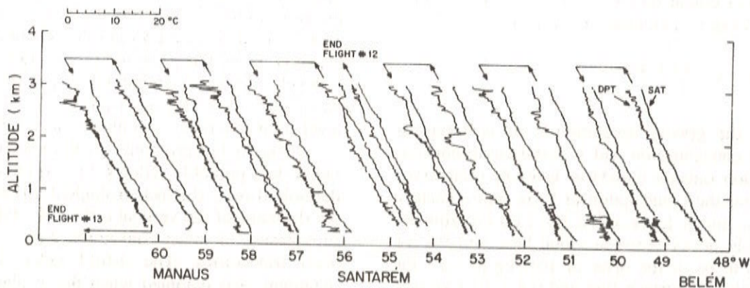
Figure 8. Dew point temperature (DPT) and static air temperature (SAT) during the trans-basin flights #12 and #13.
