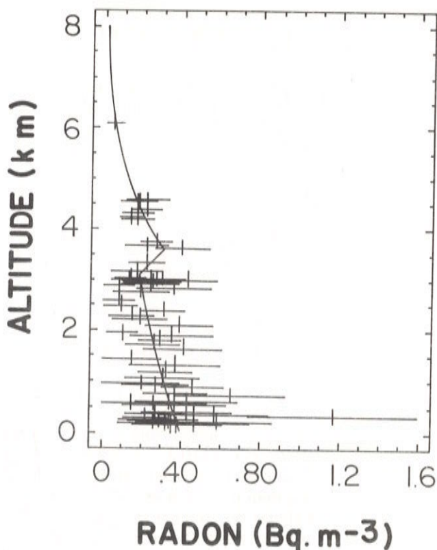
Figure 1. Radon versus geometric altitude for all leveled flights with \Delta t = 15 minutes.
