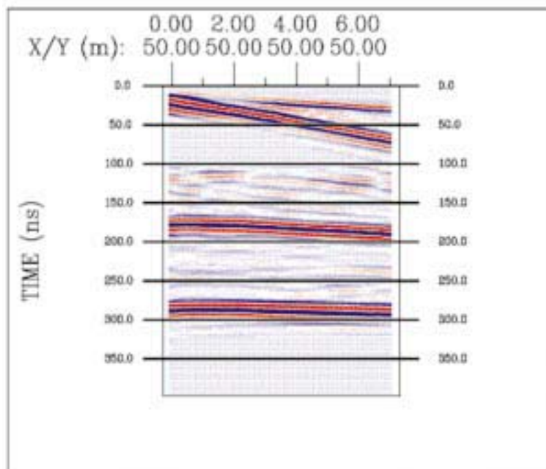
Figura 2 – Sondagem WARR adquirida com as antenas de 100MHz. Figure 2 – WARR soding acquired by 100MHz antennas.
