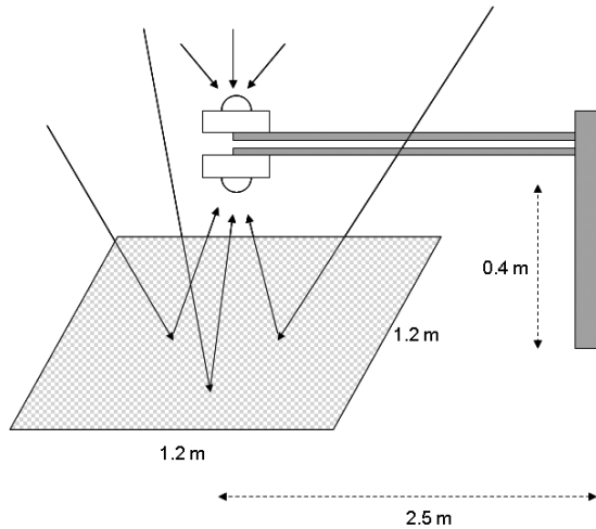
Figure 1 – Albedometer scheme.
